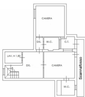
PIANO SEMINTERRATO
